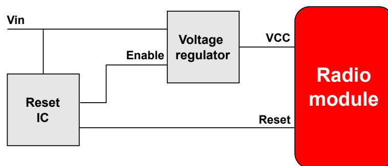
Figure 19: Reset IC
