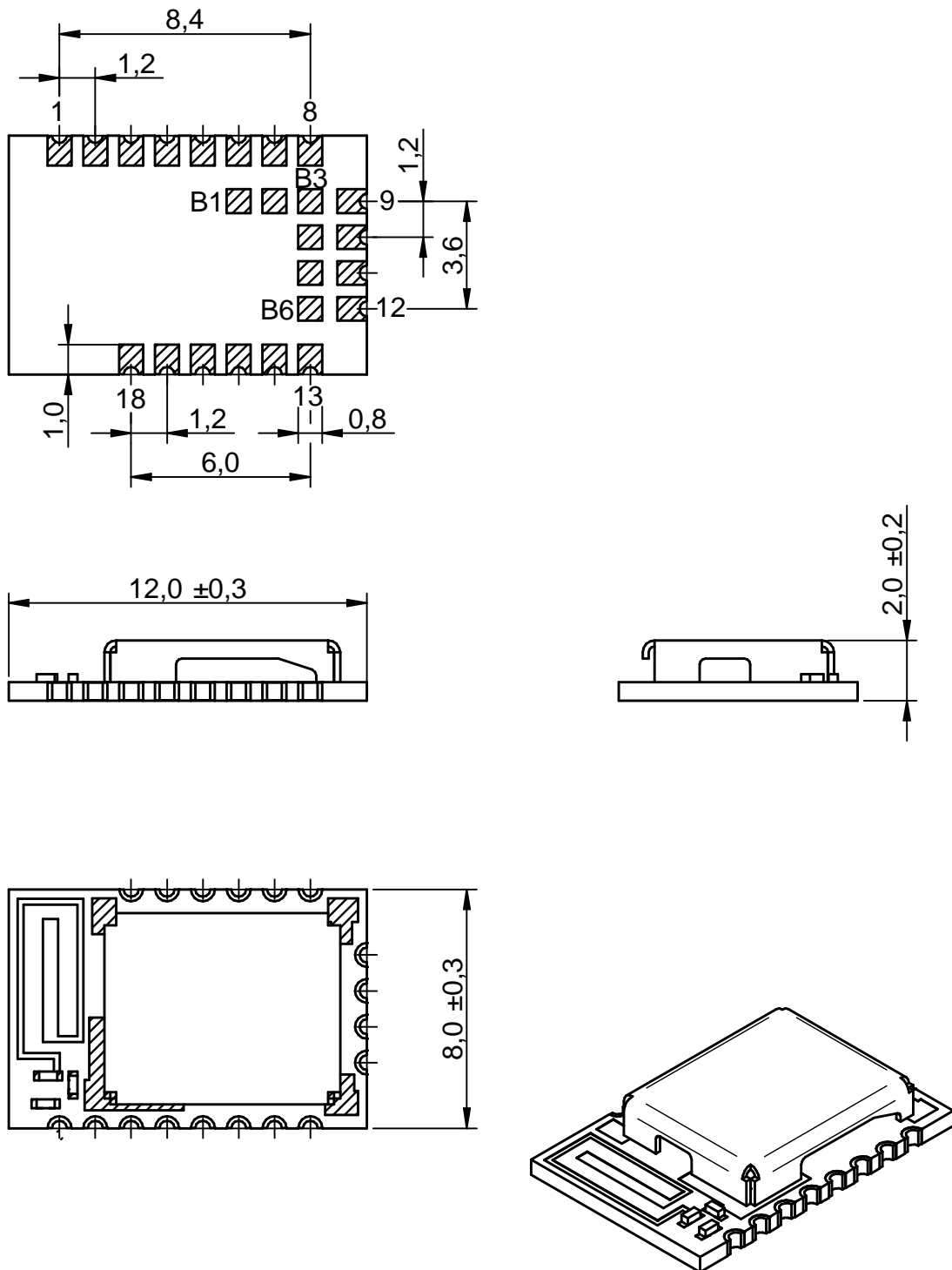
Figure 21: Module dimensions [mm]
